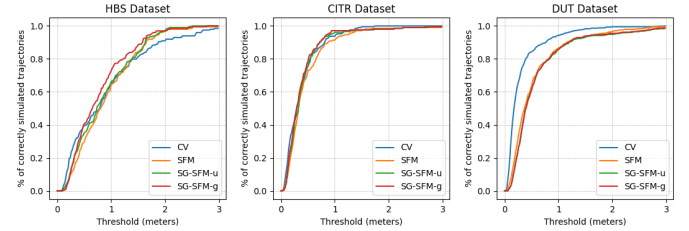
Fig. 9. Threshold of aADE vs. the percentage correctly simulated trajectory.
