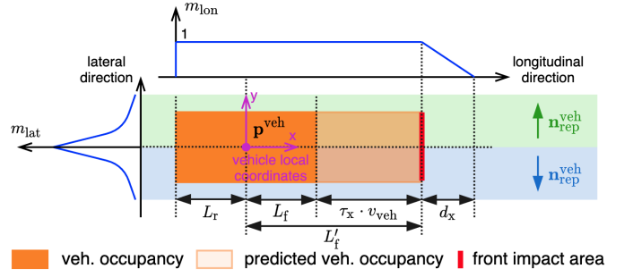
Fig. 2. Illustration of the repulsive force from a vehicle. The force direction ( \mathbf{n}_{\text{rep}}^{\text{veh}} ) points to either positive or negative y axis (green and blue arrow). The force magnitude is the multiplication of the longitudinal magnitude ( m_{\text{lon}} ) and the lateral magnitude ( m_{\text{lat}} ). See detailed description in the text.
